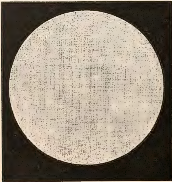
259. Appearance of the Moon when Full.
